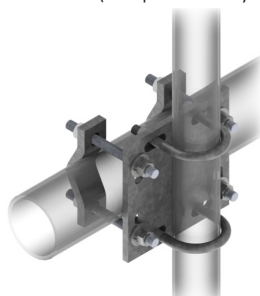
T1709KT12SA (Clamp & U-Bolt Style)
