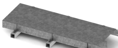
T3606KT12 8ft Long, 7in Deep 32-3/4in wide for 12 runs
